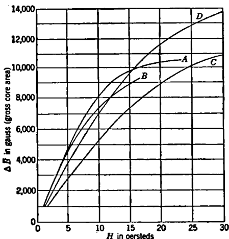
FIG. 15-9.—Loci of the tips of pulse B - H loops taken on butt-joint cores, with 1\text{-}\mu\text{sec} pulses. Curve A is for Monimax 0.003-in., \frac{1}{2} in. by \frac{1}{2} in. leg section. Curve B is for silicon Nicaloi 0.003 in., \frac{1}{2} in. by \frac{1}{2} in. leg section. Curve C is for silicon Nicaloi 0.004 in., \frac{1}{2} in. by \frac{1}{2} in. leg section. Curve D is for Hipersil 0.002 in., \frac{1}{2} in. by \frac{1}{2} in. leg section.
